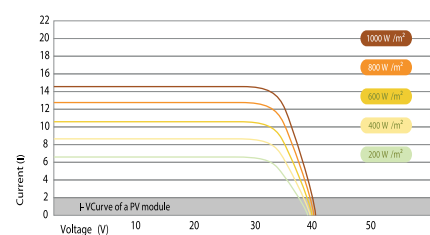
Current-Voltage Curves
